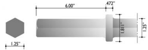
1 1/4" X 6" SHANK
