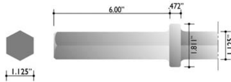
1 1/8" X 6" SHANK
